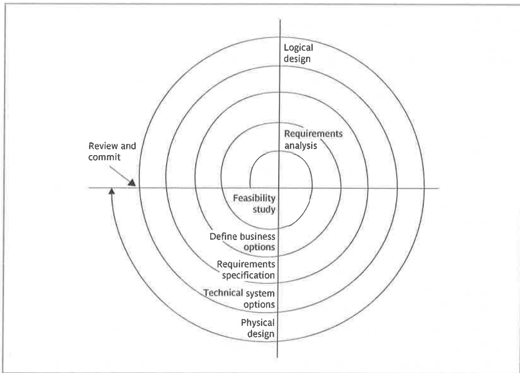
FIGURE 4.3 The application of the spiral model to SSADM version 4
