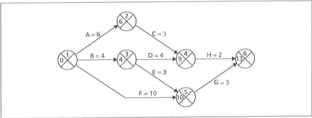
FIGURE 6.27 A CPM network after the forward pass
