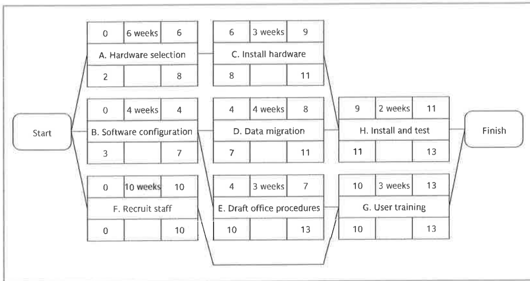
FIGURE 6.16 The network after the backward pass
