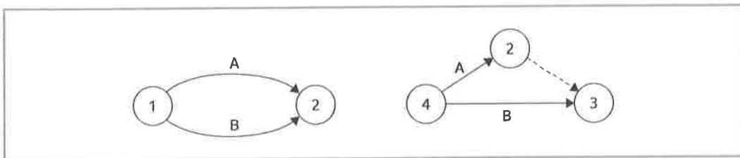
FIGURE 6.25 Another use of a dummy activity
