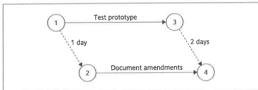
FIGURE 6.26 Using the ladder technique to indicate lags
