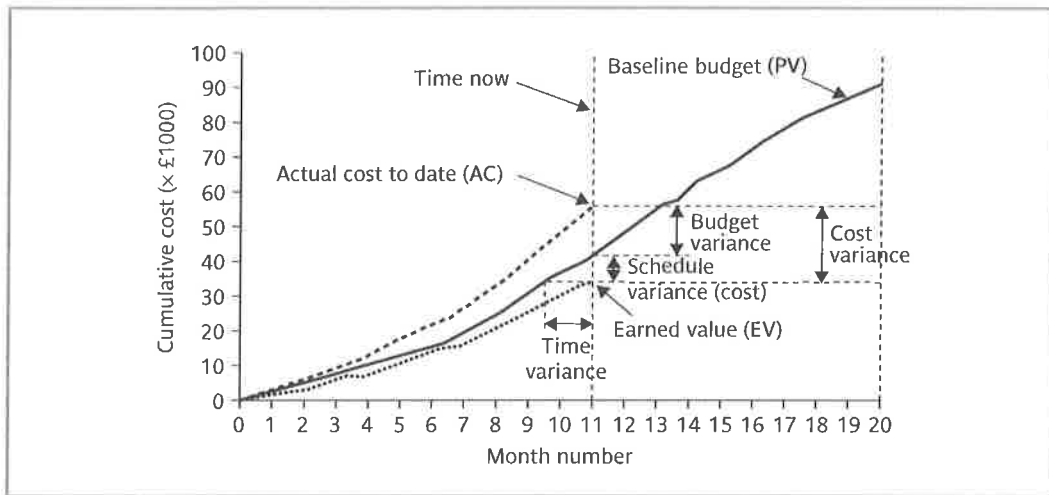
FIGURE 9.12 An earned value tracking chart
