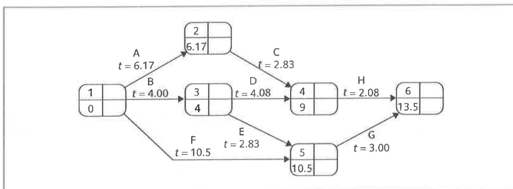
FIGURE 7.6 The PERT network after the forward pass
