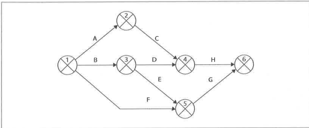
FIGURE 6.18 An activity-on-arrow network
