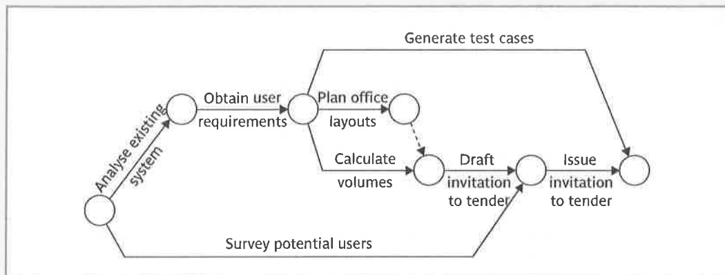
FIGURE B.6 Brigitte's CPM network
